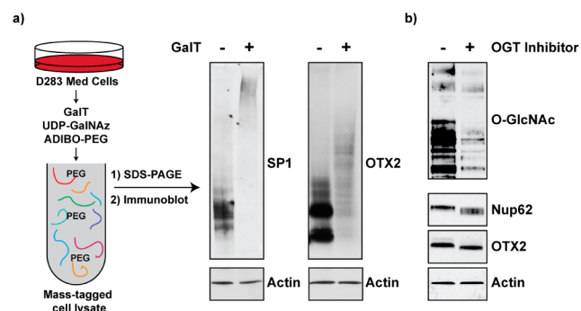
Figure 3. Endogenous OTX2 is O-GlcNAcylated in a medulloblastoma cell line. (a) Schematic of a validation method adapted from ref 21 with data shown for SP1 (positive control) and OTX2. (b) Immunoblot analysis of inhibitor-treated D283 Med cells. O-GlcNAc antibody shows decreased global O-GlcNAc, Nup62 and OTX2 show mass shifts when OGT is inhibited.
